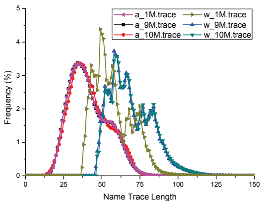
Fig. 3. Trace Length distribution 3 .
