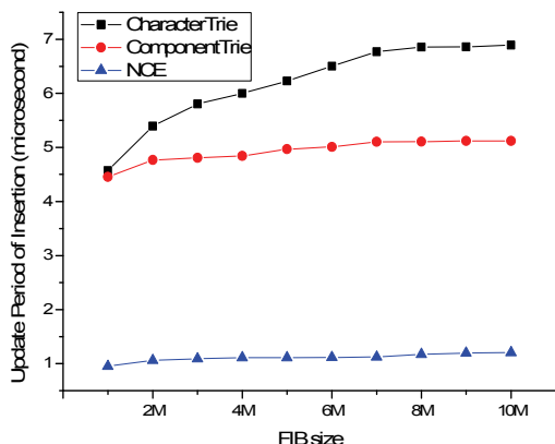
Fig. 6. The update period of insertion of the approaches on different FIB sizes.
