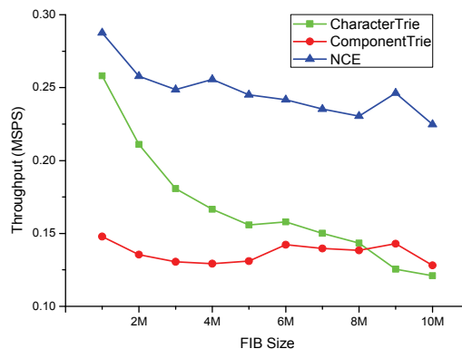
Fig. 4. The throughput of three approaches on different FIB sizes (average workload).
