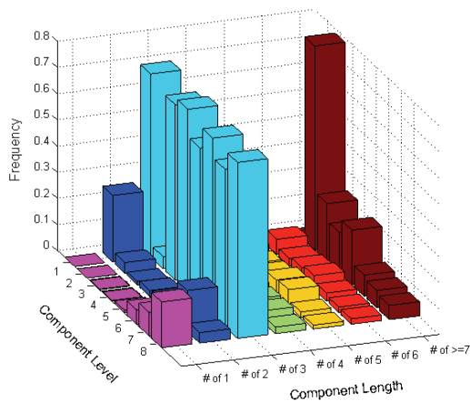
Fig. 2. The distribution of component length in each level in seed FIB.
