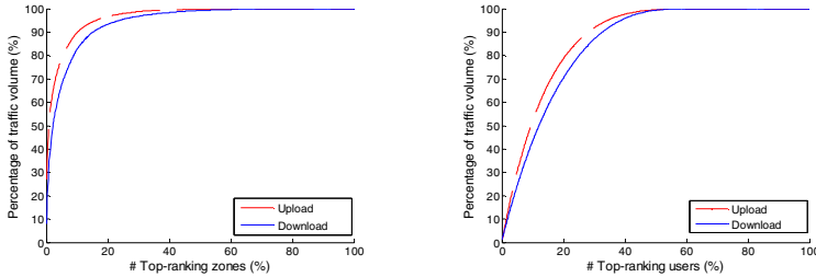
Fig. 3. The cumulative distributions of inter-zone traffic volume associated with Users / Zone level ranked in decreasing order of volume. Left: aggregate on user, Right: aggregate on zone.
